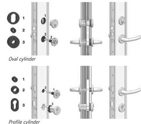
Profile cylinder
