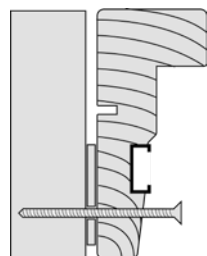
Mounting a top-hinged Daylight Window
