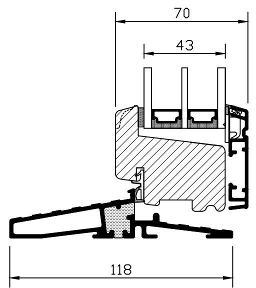
Vertical section B-B option with alu threshold
